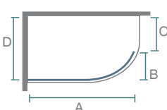
Wetroom application
